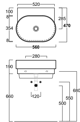
PO 06 Lavabo ovale sospeso Oval washbasin wall hung 56.47.h19
