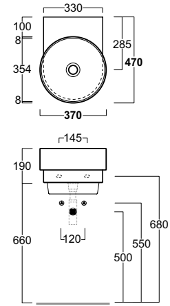
PO 05 Lavabo tondo sospeso Round washbasin wall hung Ø37.47.h19
