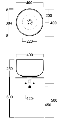
BA 02 Lavabo tondo alto d'appoggio Round countertop washbasin with high rim Ø40.h25
